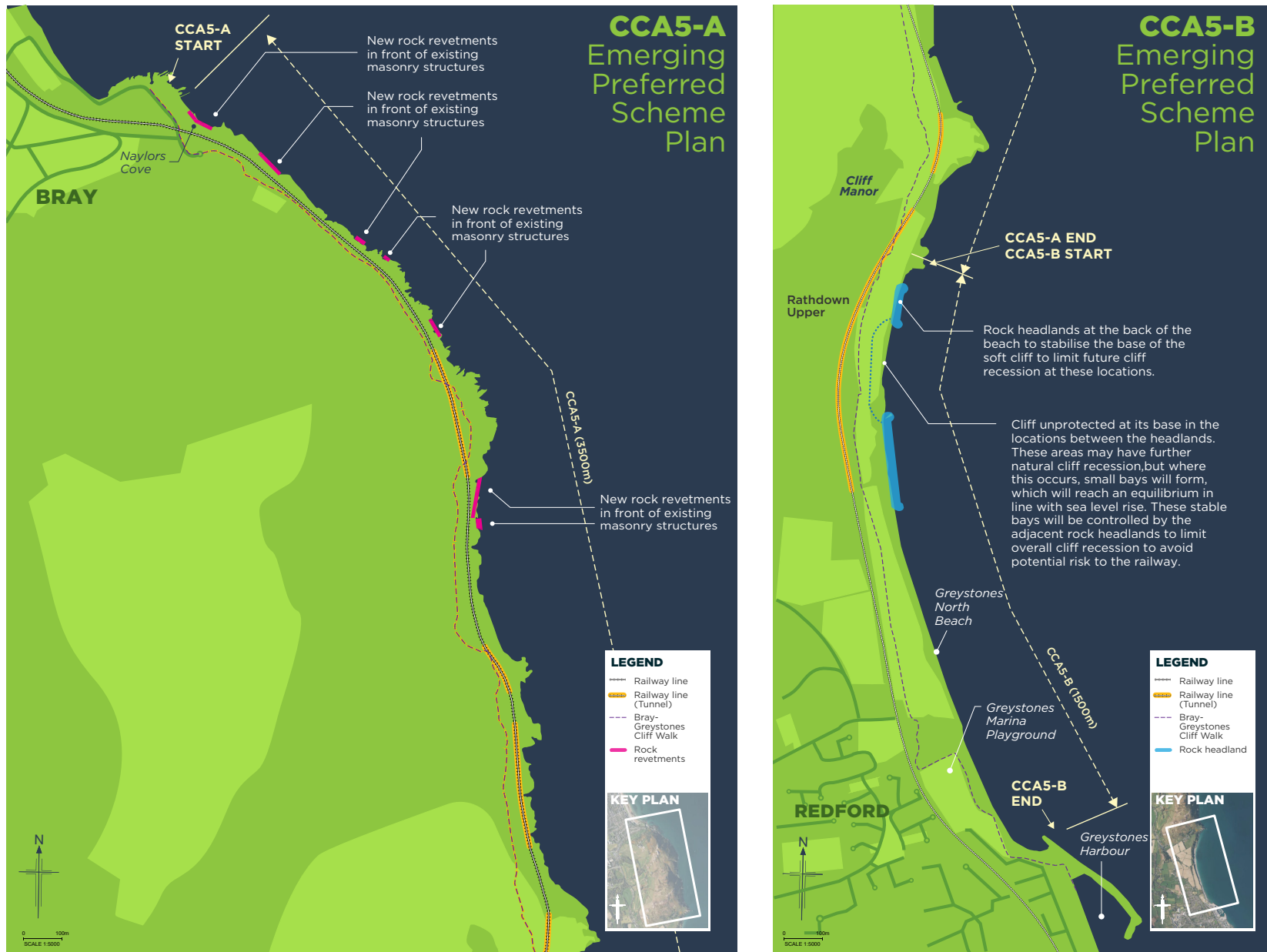
Figure 11: CCA5-A & CCA5-B Emerging Preferred Scheme Plan
