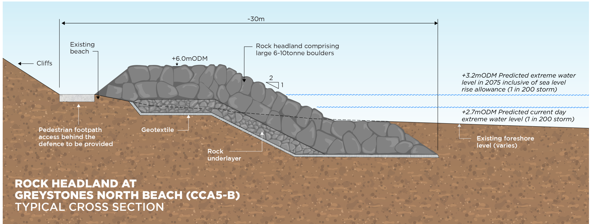
Figure 12: CCA5 Typical cross section showing rock headland trunk
