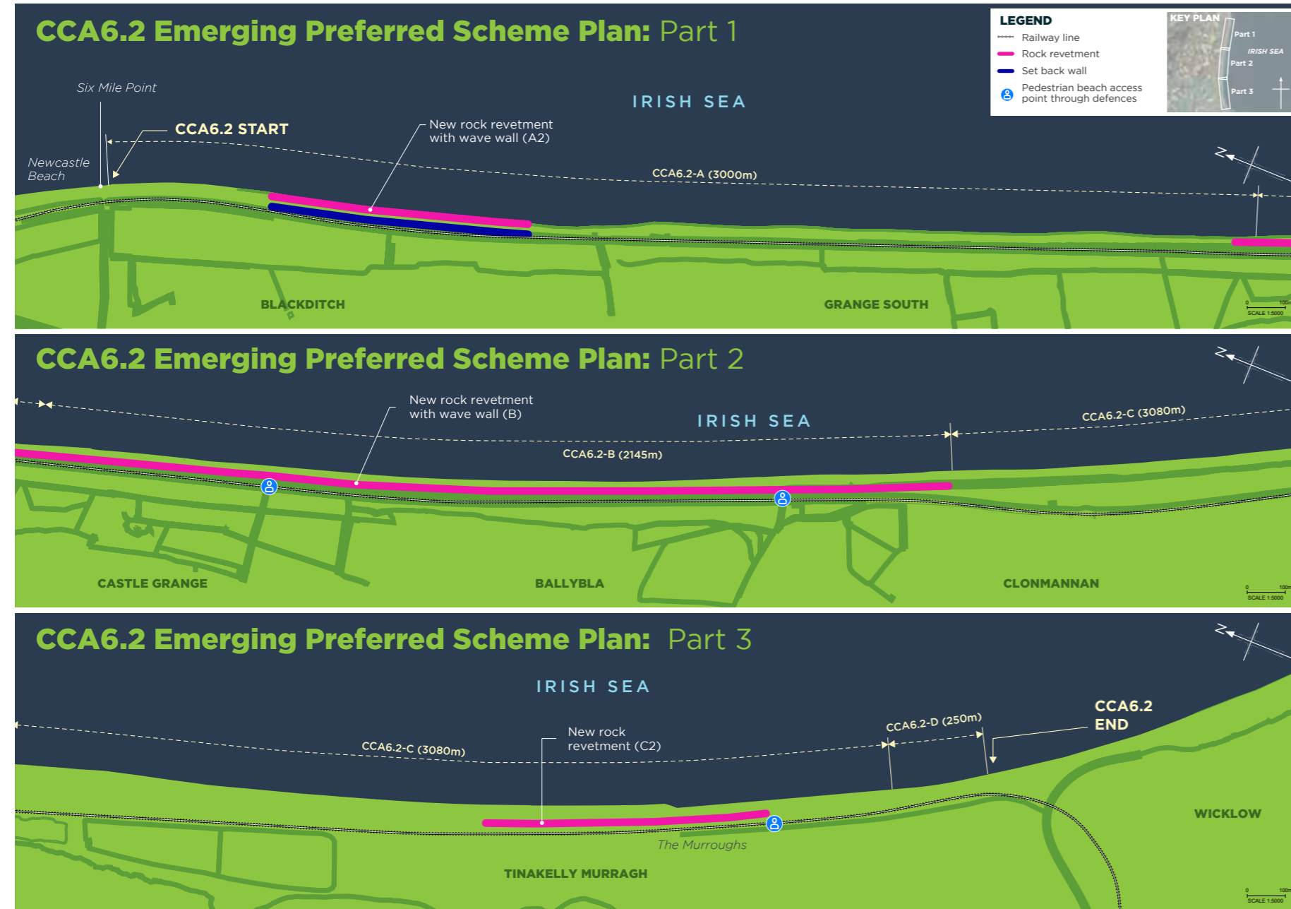
Figure 11: CCA6.2 Emerging Preferred Scheme Plan: Parts 1, 2 & 3
