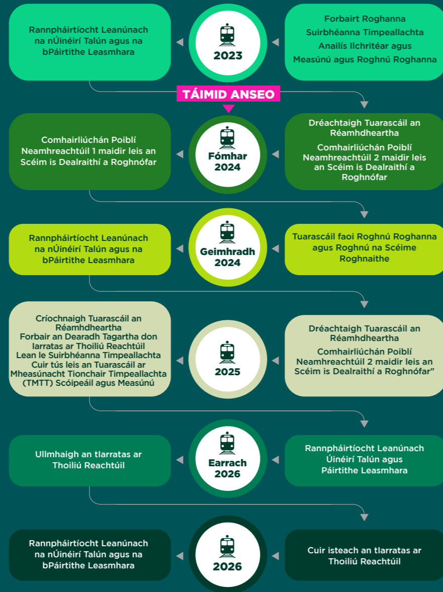
Figure 4: Consultation Roadmap
